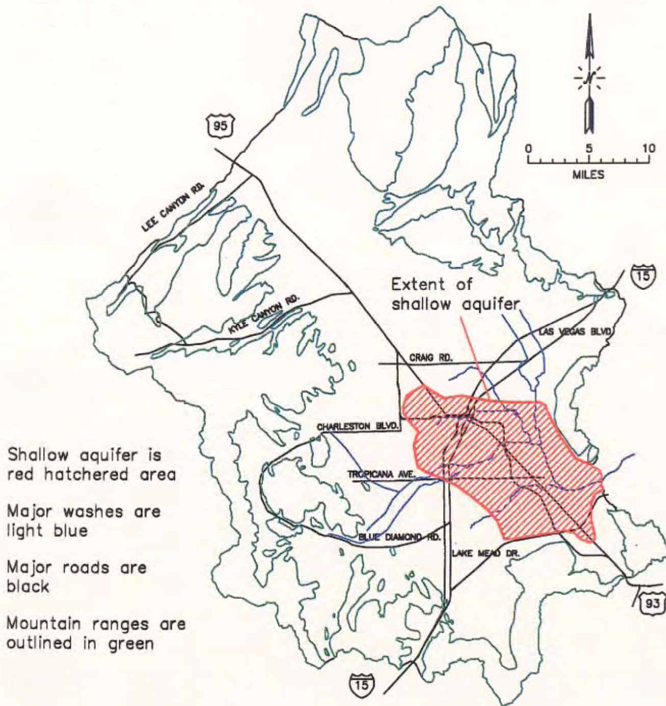
Figure 3.--Areal extent of shallow aquifer in Las Vegas Valley.
