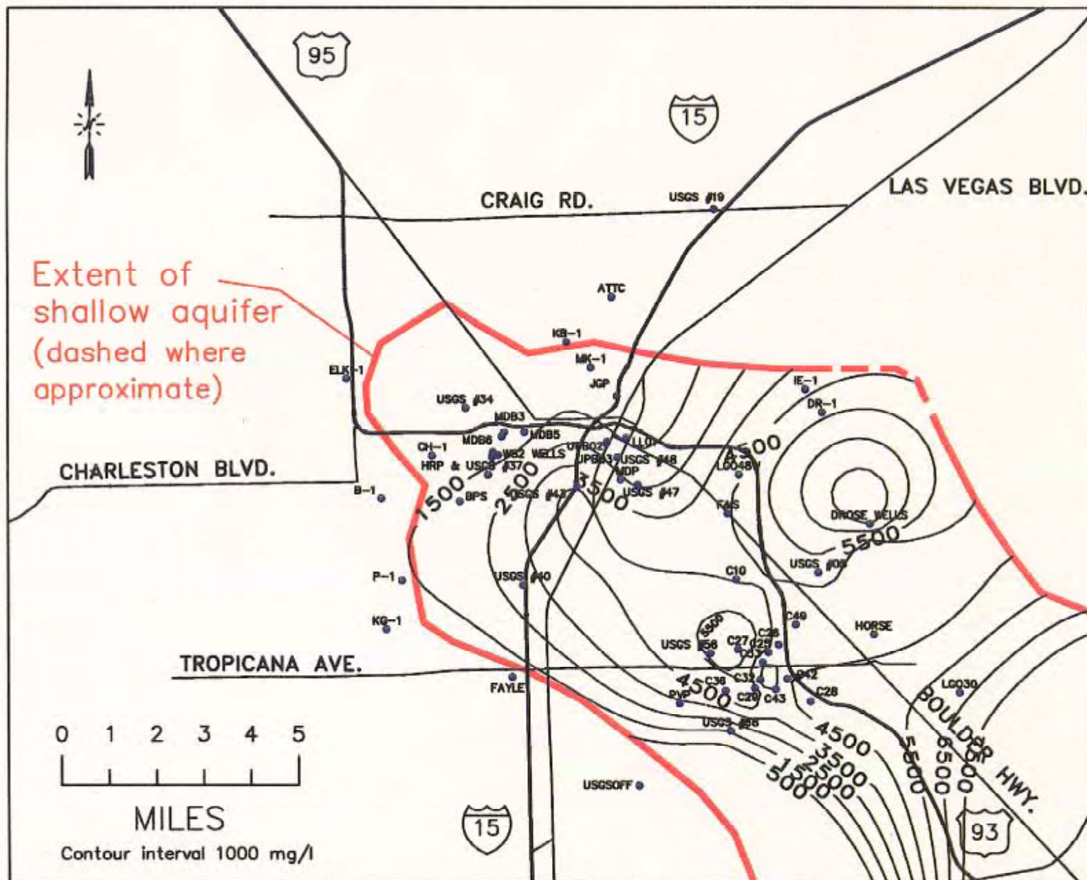
Figure 6.--Total dissolved solids contours in mg/l.
